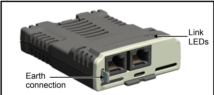
Figure 2-1 SI-Ethernet
